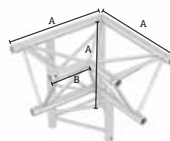
3 way corner 90° apex down left
