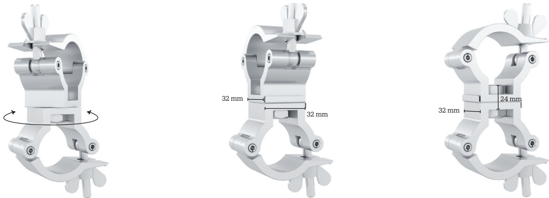
CELL134 – Swivel coupler
