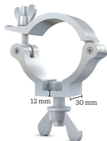
HCL5102S – Slim truss clamp with bolt + wingnut
