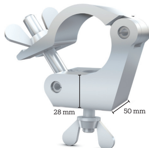
HCL 5102F – Side clamp
